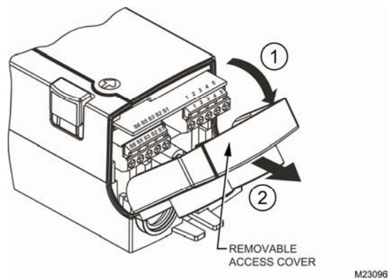
Fig. 6. Access Cover
